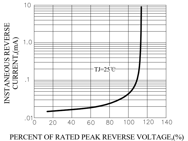
FIG.4-TYPICAL REVERSE CHARACTERISTICS
